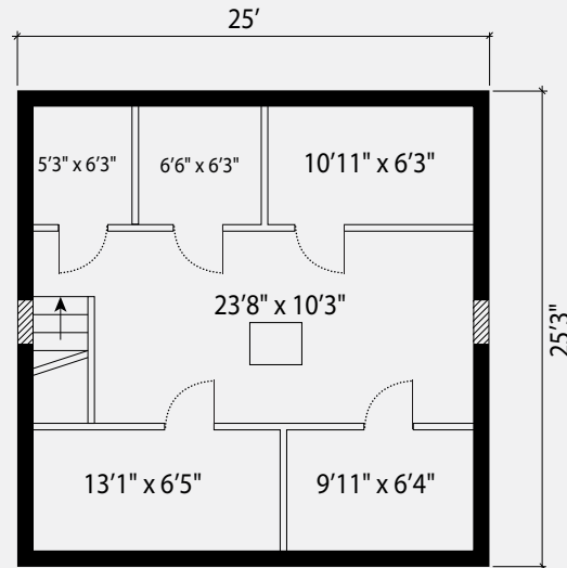
Third Floor
