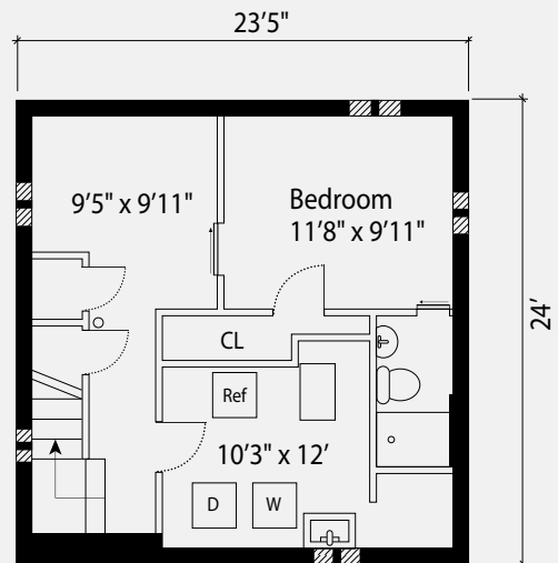
Basement
